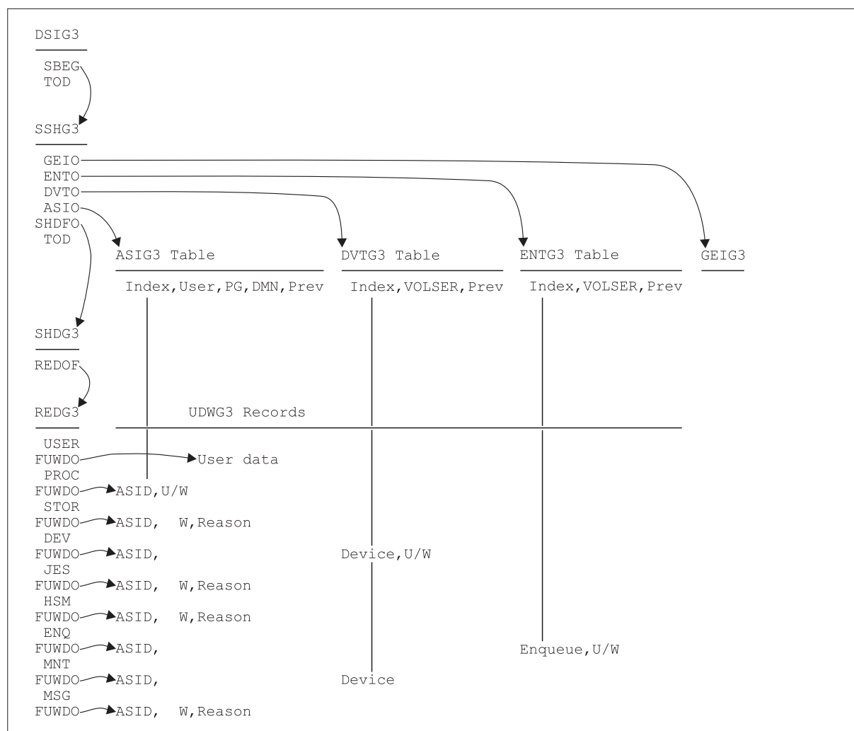
Figure 55. Monitor III Measurement Table and Record Relationships
